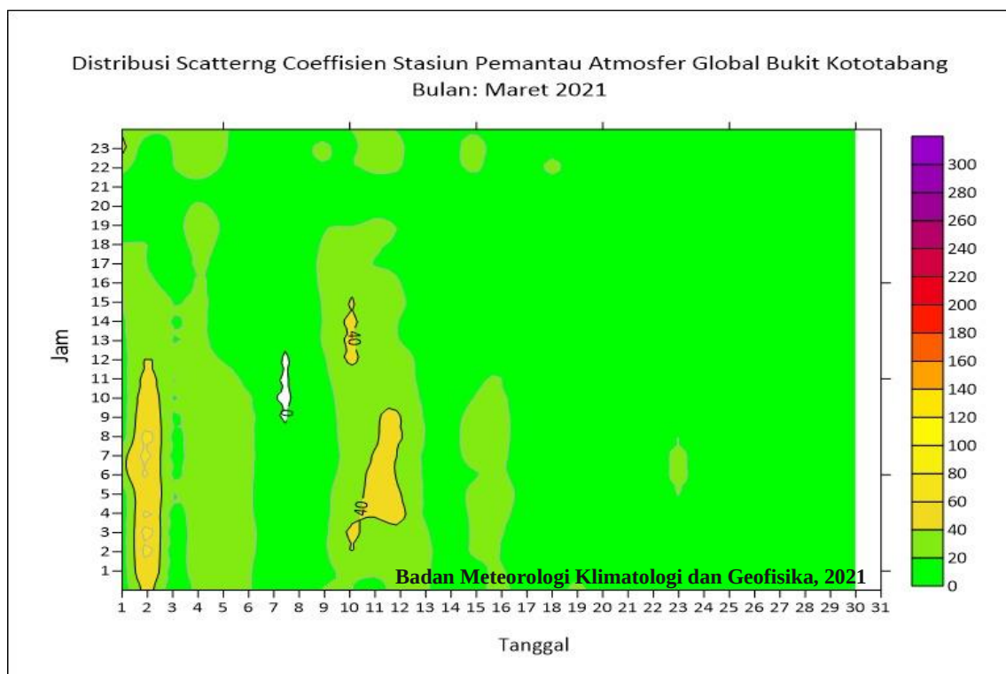
Distribusi Scattering Coefficient di Bukit Kototabang periode bulan Maret 2021
