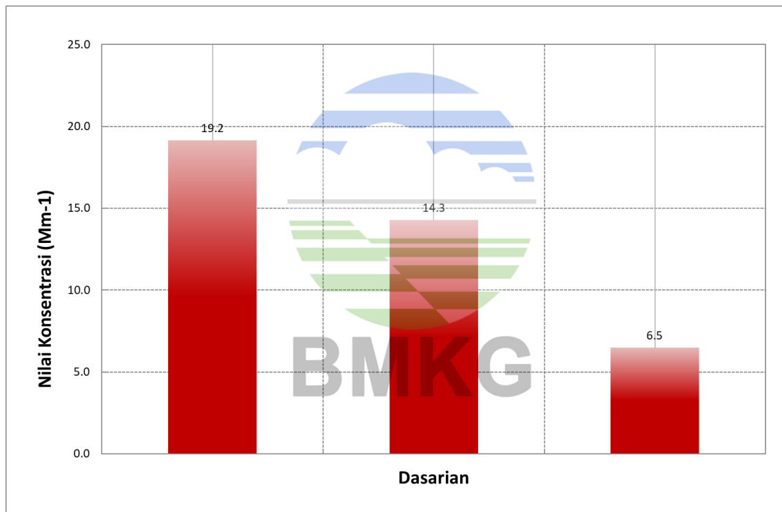
Grafik Dasarian koefisien hamburan cahaya (Scattering Coefficient) di Bukit Kototabang periode bulan Maret 2021
